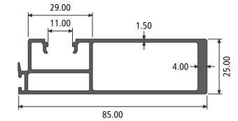
SLEEK REINFORCEMENT INTERLOCK SECTION NO. : 812858 Weight / Mtr : 1.184
