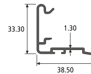
INTERLOCK SECTION NO. : 914404 Weight / Mtr : 0.350
