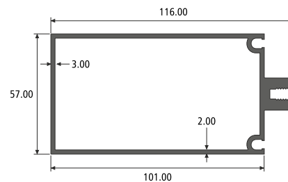
MULLION SECTION NO. : 551026 Weight / Mtr : 2.173
