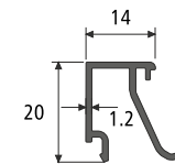
SGU CLIP SECTION NO. : 746509 Weight / Mtr : 0.202
