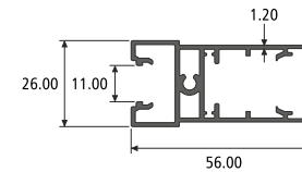
TOP & BOTTOM SECTION NO. : 992266 Weight / Mtr : 0.753
