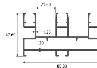
3 TRACK LIGHT SECTION NO. : 914644 Weight / Mtr : 1.420
