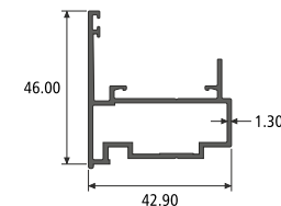
FLYING MULLION SECTION NO. : 819002 Weight / Mtr : 0.662
