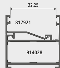
VARIOUS CLIP DETAILS
