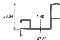
FLY MESH TRACK SECTION NO. : 914699 Weight / Mtr : 0.427
