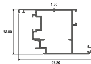
INSIDE OP. SHUTTER SECTION NO. : 992109 Weight / Mtr : 1.540
