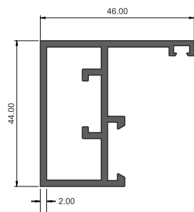
STILE DOOR - FRAME PROFILE
