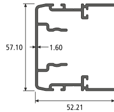
DOUBLE INTERLOCK SECTION NO. : 817088 Weight / Mtr : 1.055
