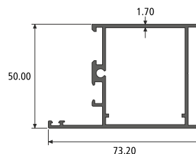
FRAME SECTION NO. : 914775 Weight / Mtr : 1.080
