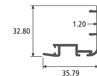
MOSQUITO INTERLOCK SECTION NO. : 955368 Weight / Mtr : 0.310
