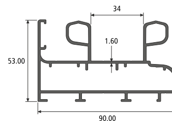
2 TRACK WITH LEG SECTION NO. : 955077 Weight / Mtr : 1.819
