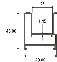
2 TRACK SECTION NO. : 914036 Weight / Mtr : 0.873
