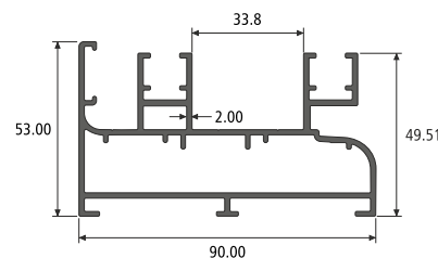
2 TRACK WITH LEG SECTION NO. : 551015 Weight / Mtr : 1.822
