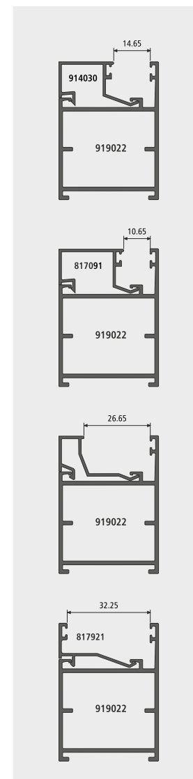
VARIOUS CLIP DETAILS
