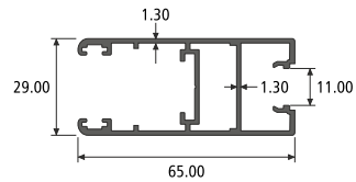
SGU SHUTTER SECTION NO. : 914405 Weight / Mtr : 0.890
