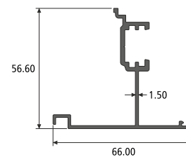
FLYING MULLION SECTION NO. : 914797 Weight / Mtr : 0.707
