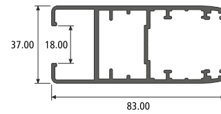
LAMINATED GLASS SHUTTER SECTION NO. : 992173 Weight / Mtr : 1.450
