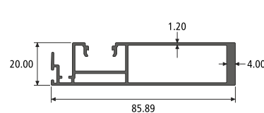
REINFORCEMENT INTERLOCK SECTION NO. : 992268 Weight / Mtr : 0.975
