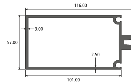
MULLION SECTION NO. : 551027 Weight / Mtr : 2.641
