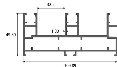
3 TRACK SECTION NO. : 812514 Weight / Mtr : 2.309
