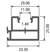
SLEEK INTERLOCK SECTION NO. : 992324 Weight / Mtr : 0.524
