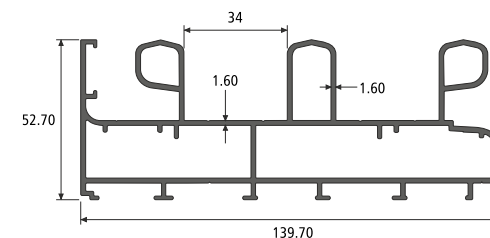
3 TRACK WITH LEG SECTION NO. : 967067 Weight / Mtr : 2.675
