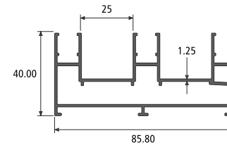
3 TRACK SECTION NO. : 955389 Weight / Mtr : 1.240
