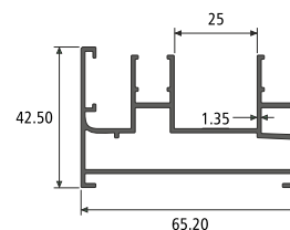
2 TRACK SECTION NO. : 955388 Weight / Mtr : 0.795
