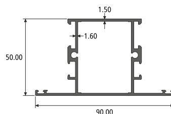
MULLION SECTION NO. : 914774 Weight / Mtr : 1.235
