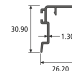
INTERLOCK SECTION NO. : 551025 Weight / Mtr : 0.230
