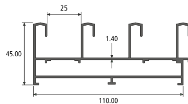
4 TRACK SECTION NO. : 812536 Weight / Mtr : 1.765
