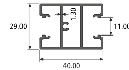
MIDDLE SECTION NO. : 817032 Weight / Mtr : 0.672
