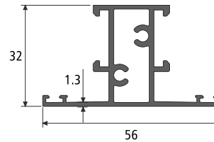
MULLION SECTION NO. : 819081 Weight / Mtr : 0.694
