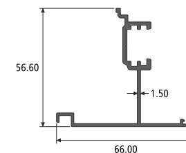
FLYING MULLION SECTION NO. : 914797 Weight / Mtr : 0.707
