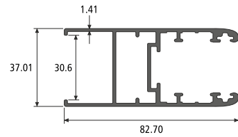
DGU SHUTTER SECTION NO. : 914409 Weight / Mtr : 1.274
