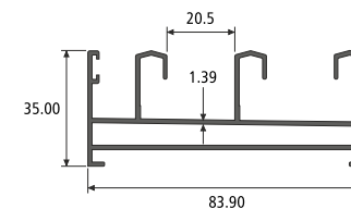
3 TRACK SECTION NO. : 551024 Weight / Mtr : 1.130
