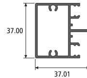
MOSQUITO MIDDLE SECTION NO. : 817089 Weight / Mtr : 0.673
