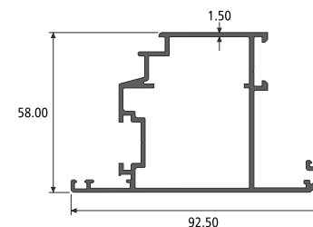
OUTSIDE OP. SHUTTER (SINGLE POINT LOCKING) SECTION NO. : 914776 Weight / Mtr : 1.292
