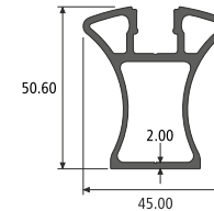
REINFORCEMENT PROFILE SECTION NO. : 914806 Weight / Mtr : 1.104
