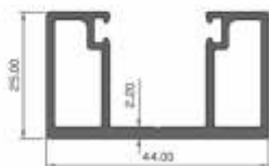
FIXED PROFILE
