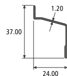
RAIN TRACK SECTION NO. : 817061 Weight / Mtr : 0.195
