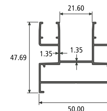
2 TRACK LIGHT SECTION NO. : 914643 Weight / Mtr : 0.865
