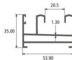
2 TRACK SECTION NO. : 551023 Weight / Mtr : 0.800
