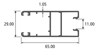
MOSQUITO SHUTTER LIGHT SECTION NO. : 914900 Weight / Mtr : 0.705
