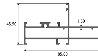
BIG FRAME SECTION NO. : 914756 Weight / Mtr : 1.185
