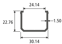
LAMINATED GLASS ADAPTOR SECTION NO. : 992087 Weight / Mtr : 0.297
