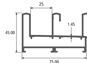
3 TRACK SECTION NO. : 955069 Weight / Mtr : 1.405
