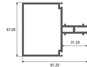
TRANSOM SECTION NO. : 551011 Weight / Mtr : 1.659
