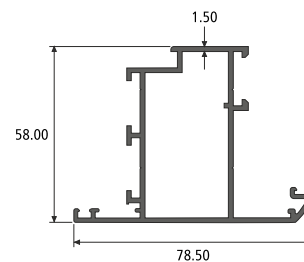
OUTSIDE OP. SHUTTER SECTION NO. : 914353 Weight / Mtr : 1.138
