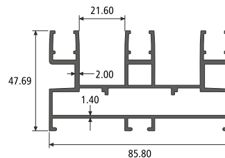
3 TRACK SECTION NO. : 914402 Weight / Mtr : 1.724
