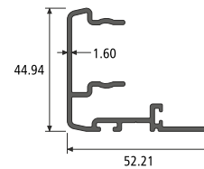
INTERLOCK SECTION NO. : 955110 Weight / Mtr : 0.689
