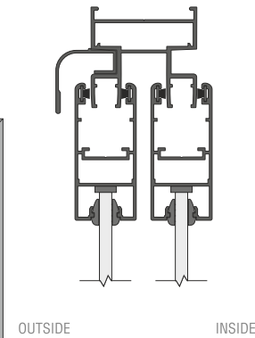
29mm SLEEK TWO TRACK TWO SHUTTER ASSEMBLY
