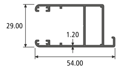
MOSQUITO SHUTTER SECTION NO. : 914698 Weight / Mtr : 0.617
