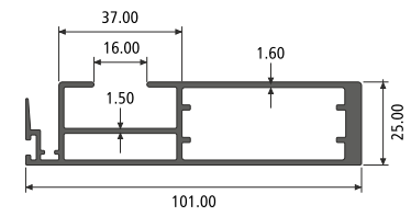
SLEEK REINFORCEMENT INTERLOCK SECTION NO. : 812859 Weight / Mtr : 1.472
