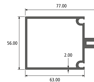
TRANSOM SECTION NO. : 812958 Weight / Mtr : 1.591
