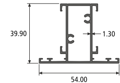
MULLION SECTION NO. : 819006 Weight / Mtr : 0.715
