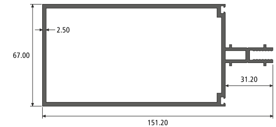
MULLION SECTION NO. : 551010 Weight / Mtr : 2.896
