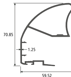
REINFORCEMENT INTERLOCK SECTION NO. : 817034 Weight / Mtr : 0.920
