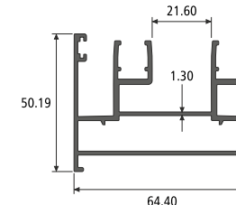
2 TRACK WITH LEG SECTION NO. : 812520 Weight / Mtr : 1.325
