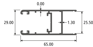
DGU SHUTTER SECTION NO. : 914897 Weight / Mtr : 0.796
