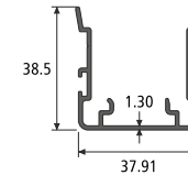
DOUBLE INTERLOCK SECTION NO. : 817086 Weight / Mtr : 0.528
