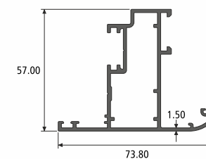
SHUTTER SECTION NO. : 992178 Weight / Mtr : 1.100
