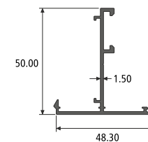
INVERSION SECTION NO. : 914564 Weight / Mtr : 0.508
