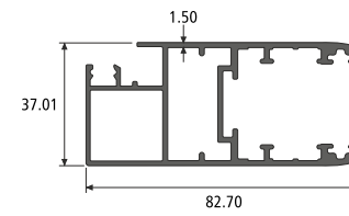
MOSQUITO SHUTTER SECTION NO. : 992086 Weight / Mtr : 1.397
