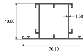
BIG SHUTTER SECTION NO. : 819013 Weight / Mtr : 0.867
