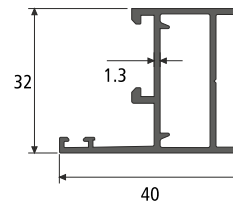
FRAME SECTION NO. : 745611 Weight / Mtr : 0.449
