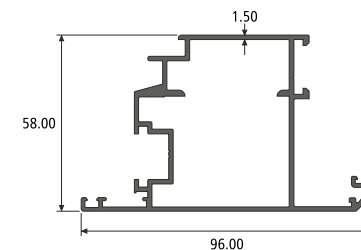
OUTSIDE OP. SHUTTER (MULTI POINT LOCKING) SECTION NO. : 992214 Weight / Mtr : 1.402
