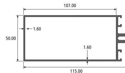
TRANSOM SECTION NO. : 551037 Weight / Mtr : 1.596
