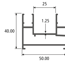
2 TRACK SECTION NO. : 955388 Weight / Mtr : 0.795
