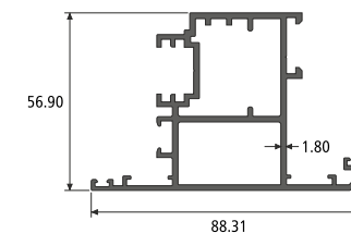
SHUTTER SECTION NO. : 992166 Weight / Mtr : 1.623
