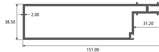
HALF MULLION SECTION NO. : 551012 Weight / Mtr : 2.061
