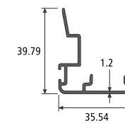
INTERLOCK SECTION NO. : 955391 Weight / Mtr : 0.370
