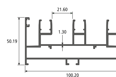
3 TRACK WITH LEG SECTION NO. : 551009 Weight / Mtr : 1.969
