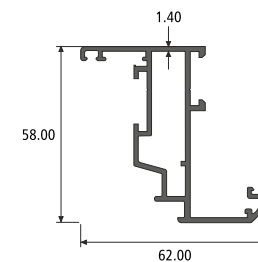
INSIDE OP. SHUTTER SECTION NO. : 914520 Weight / Mtr : 0.955
