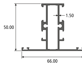
MULLION SECTION NO. : 914352 Weight / Mtr : 1.015
