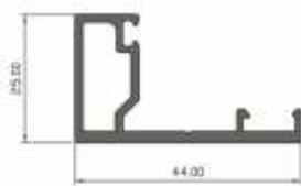
BOTTOM PROFILE
