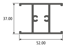
INTERMEDIATE SHUTTER SECTION NO. : 992091 Weight / Mtr : 0.957
