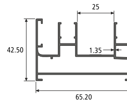
2 TRACK SECTION NO. : 955388 Weight / Mtr : 0.795
