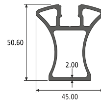
REINFORCEMENT PROFILE SECTION NO. : 914806 Weight / Mtr : 1.104
