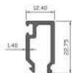
CLIP ON PROFILE
