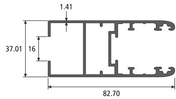
SGU SHUTTER SECTION NO. : 914668 Weight / Mtr : 1.335
