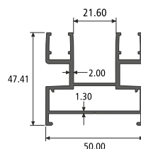
2 TRACK SECTION NO. : 914400 Weight / Mtr : 1.100
