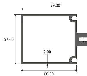
TRANSOM SECTION NO. : 812957 Weight / Mtr : 1.787
