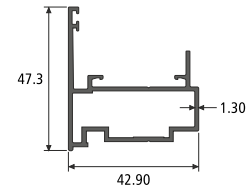
FLING MULLION SECTION NO. : 819002 Weight / Mtr : 0.662
