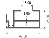
SLEEK INTERLOCK SECTION NO. : 992326 Weight / Mtr : 0.676
