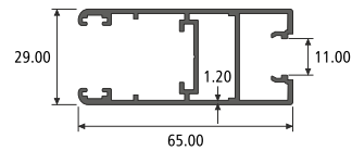
SGU SHUTTER LIGHT SECTION NO. : 914642 Weight / Mtr : 0.815
