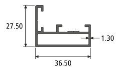
SASH SECTION NO. : 992003 Weight / Mtr : 0.470
