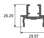
MATING PROFILE INSERTED COUNTER PLATE SECTION NO. : 992148 Weight / Mtr : 0.478
