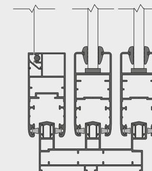
37mm FLYMESH
