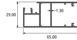
MOSQUITO SHUTTER SECTION NO. : 992222 Weight / Mtr : 0.816
