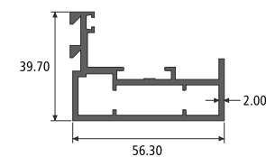
SHUTTER SECTION NO. : 992097 Weight / Mtr : 1.106
