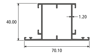
BIG SHUTTER SECTION NO. : 914891 Weight / Mtr : 0.755
