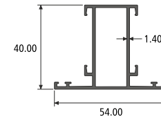
INSIDE / OUTSIDE SHUTTER SECTION NO. : 914890 Weight / Mtr : 0.660
