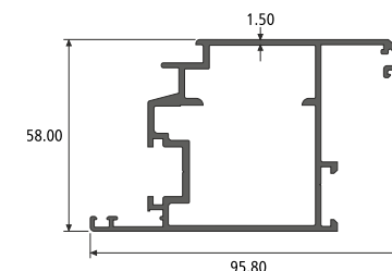
INSIDE OP. SHUTTER SECTION NO. : 992109 Weight / Mtr : 1.540
