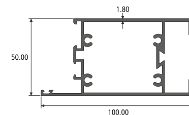
DOOR BOTTOM SECTION NO. : 914777 Weight / Mtr : 1.766
