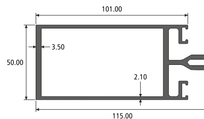
MULLION SECTION NO. : 551038 Weight / Mtr : 2.505
