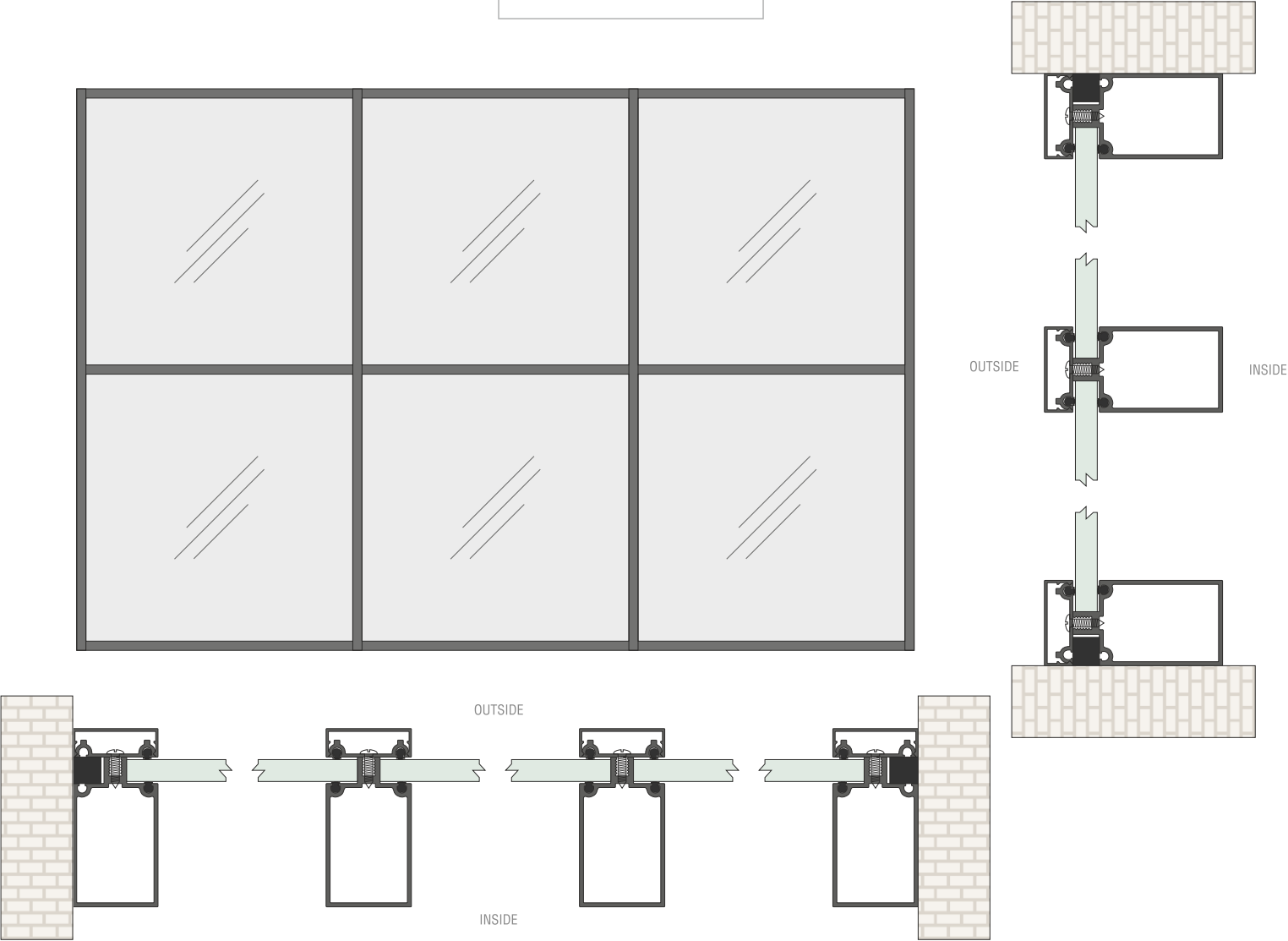
45mm CURTAIN WALL
