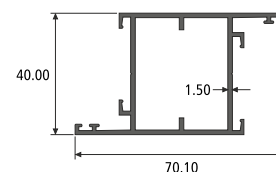
Z MULLION SHUTTER SECTION NO. : 819021 Weight / Mtr : 0.870
