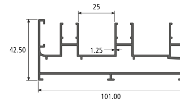
3 TRACK SECTION NO. : 955389 Weight / Mtr : 1.240
