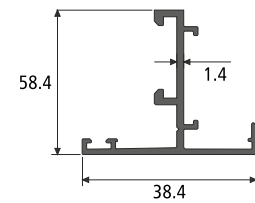
INVERSION PROFILE SECTION NO. : 746510 Weight / Mtr : 0.369
