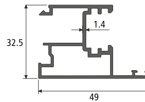
FLYING MULLION SECTION NO. : 819082 Weight / Mtr : 0.623
