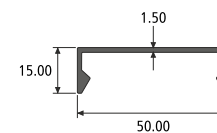
COVER PLATE SECTION NO. : 551042 Weight / Mtr : 0.365
