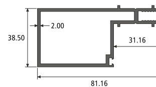
HALF TRANSOM SECTION NO. : 819503 Weight / Mtr : 1.294
