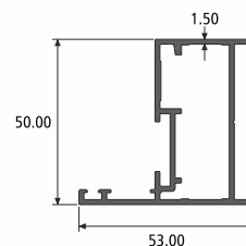
FRAME SECTION NO. : 992177 Weight / Mtr : 0.882
