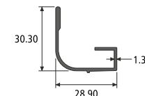
RAIN TRACK SECTION NO. : 914519 Weight / Mtr : 0.283
