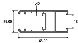
SHUTTER FOR LAMINATED GLASS SECTION NO. : 992111 Weight / Mtr : 0.890
