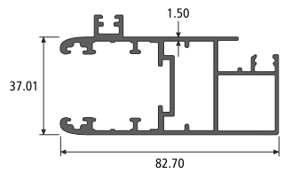
MOSQUITO SHUTTER WITH WOOLPILE SEALING GROOVE SECTION NO. : 812676 Weight / Mtr : 1.518
