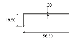
COVER CAP SECTION NO. : 812960 Weight / Mtr : 0.321
