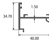
INVERSION SECTION NO. : 819014 Weight / Mtr : 0.433
