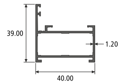
FRAME SECTION NO. : 914028 Weight / Mtr : 0.547
