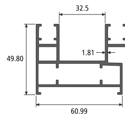
2 TRACK SECTION NO. : 992248 Weight / Mtr : 1.431
