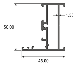
FRAME SECTION NO. : 914351 Weight / Mtr : 0.818
