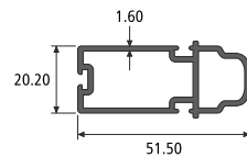
MATING PROFILE FRONT FITTED COUNTER PLATE SECTION NO. : 817072 Weight / Mtr : 0.720
