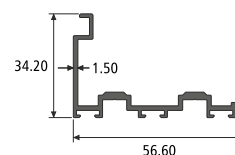
DOOR BOTTOM ADAPTOR SECTION NO. : 992208 Weight / Mtr : 0.526
