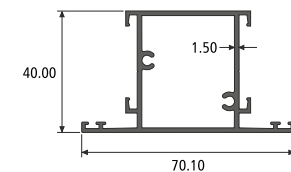
MULLION SECTION NO. : 819008 Weight / Mtr : 0.905
