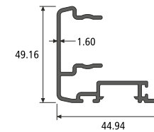
INTERLOCK SECTION NO. : 992312 Weight / Mtr : 0.693
