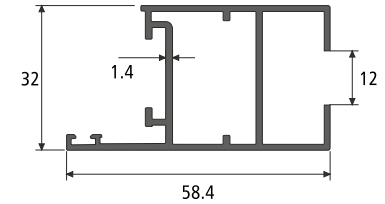
IN / OUT OPENABLE SHUTTER SECTION NO. : 819080 Weight / Mtr : 0.726
