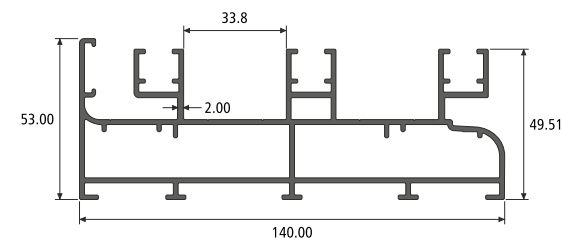
3 TRACK WITH LEG SECTION NO. : 551016 Weight / Mtr : 2.688
